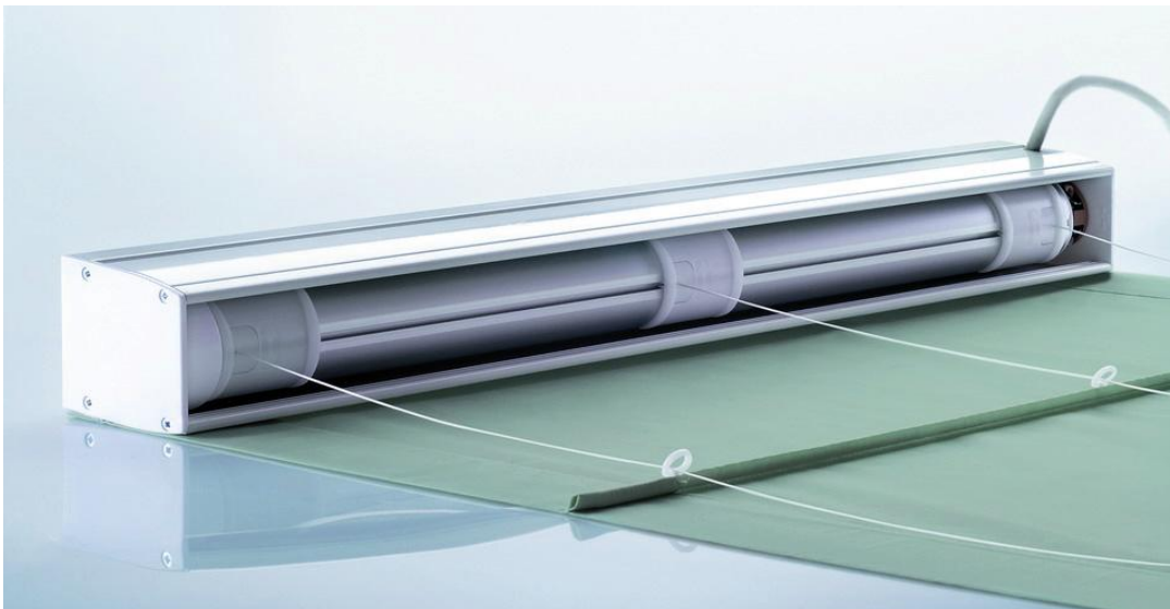
The system Silent Gliss 2350 is composed of a single cassette and very few parts which allow easy assembling and installation.
